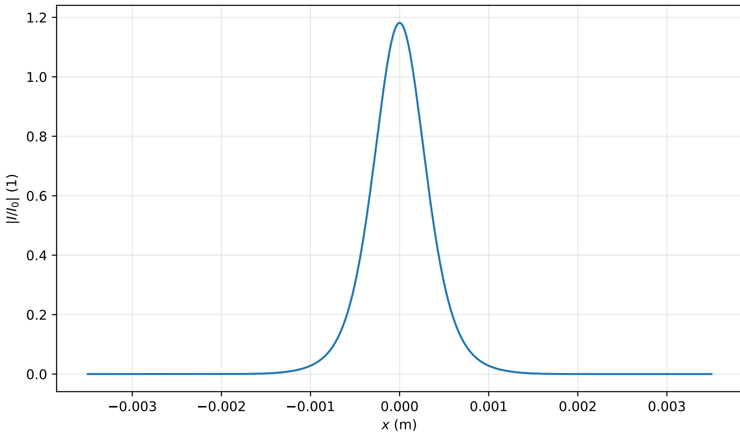
Intensity profile I(x, y = 0, z = 1.592m)/I_0 , P_{in}=0.7P_{cr} , artificial time
